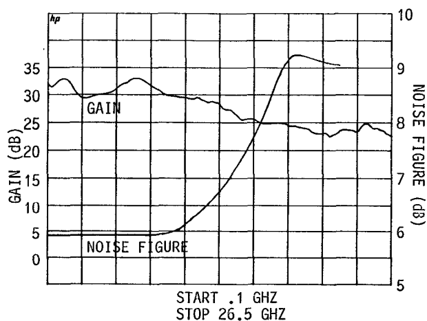
Figure 3. Gain and noise figure for the 4 stage amplifier cascade over the 100-MHz to 22-GHz frequency range.
